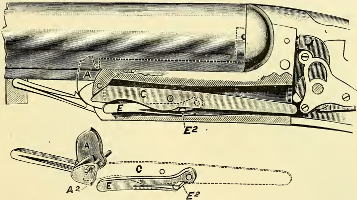
Southgate's Ejecting Mechanism and Separate Limbs.
